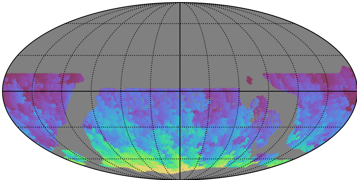
too_10_1v3.4_10yrs WFD r band: Max HA
