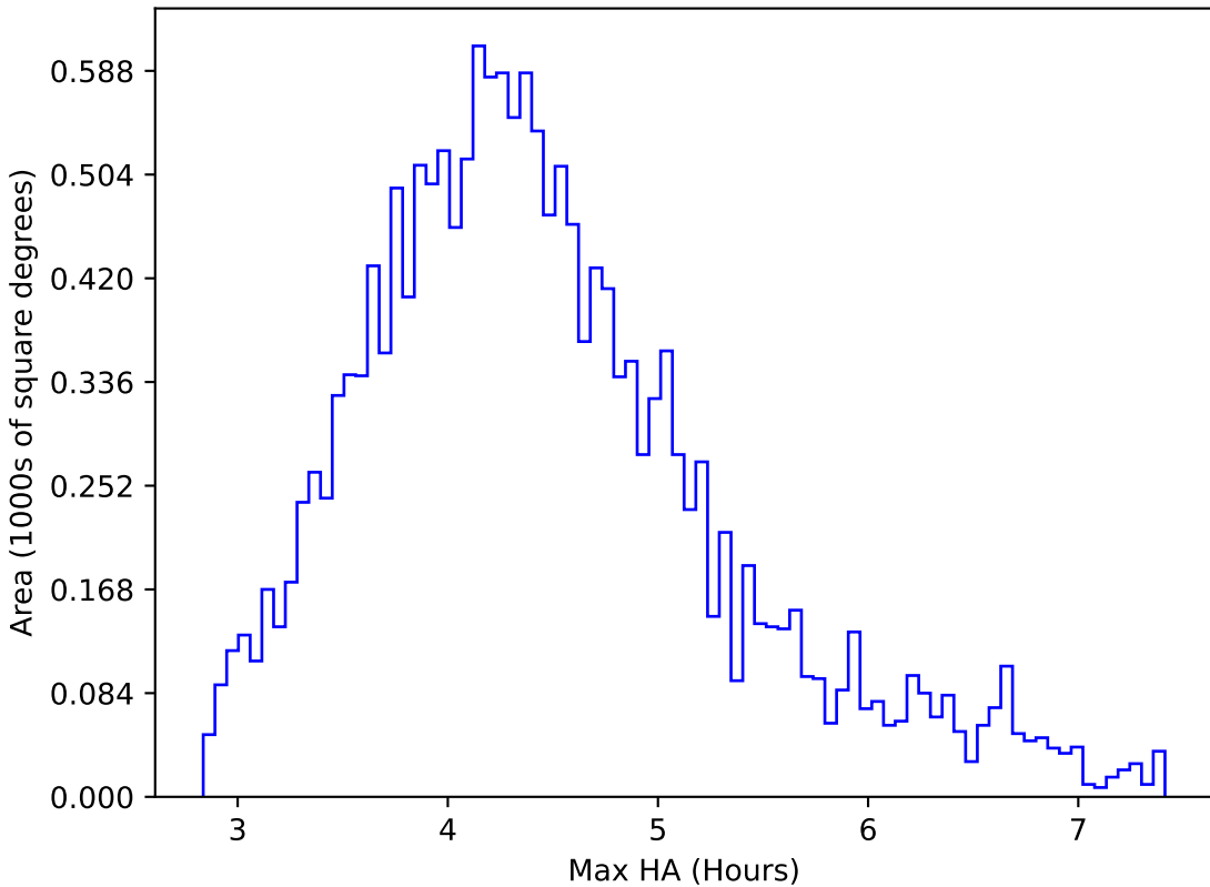
too_10_1v3.4_10yrs WFD r band: Max HA
