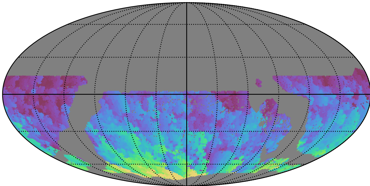
too_10_1v3.4_10yrs WFD g band: Max HA
