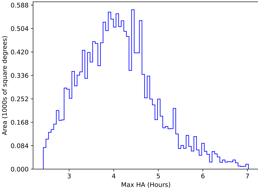
too_10_1v3.4_10yrs WFD g band: Max HA
