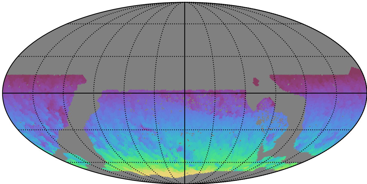
too_10_1v3.4_10yrs WFD all bands: Max HA
