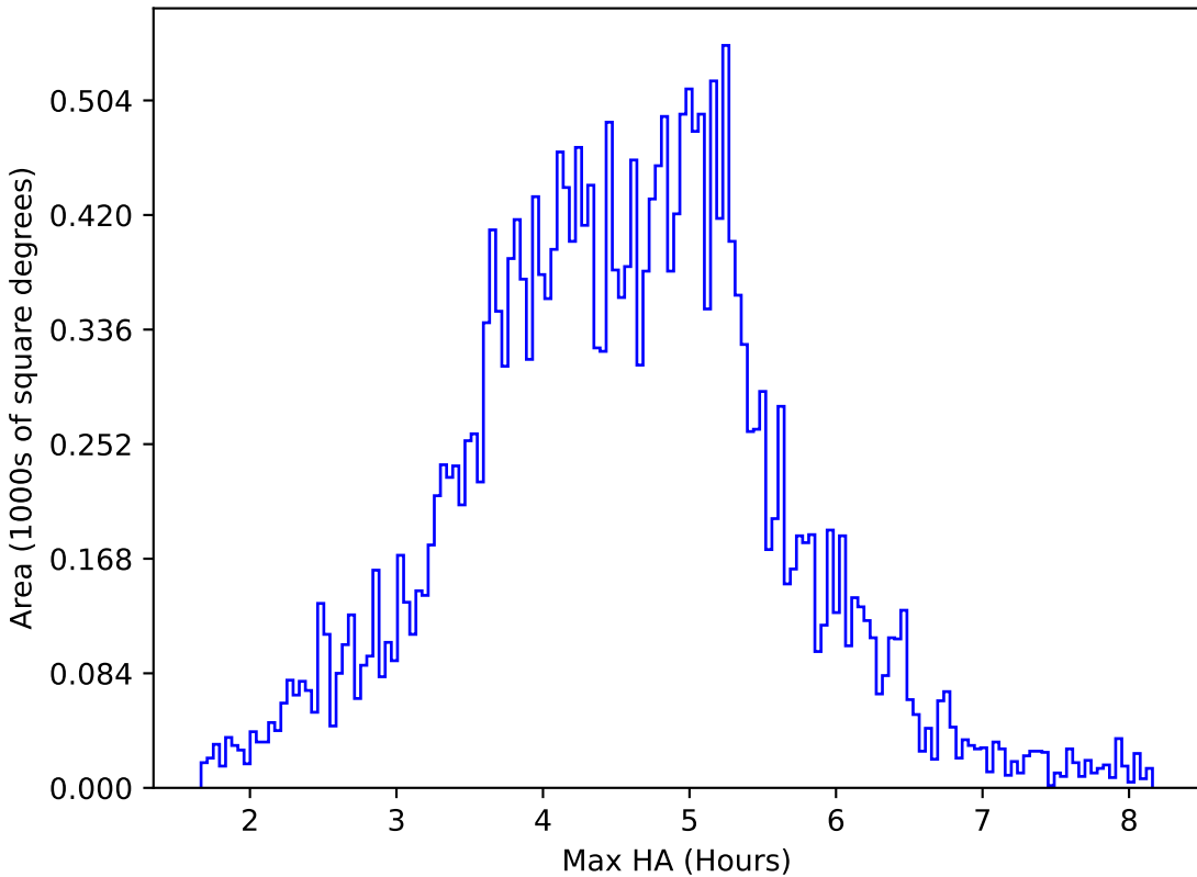
too_10_1v3.4_10yrs All sky z band: Max HA
