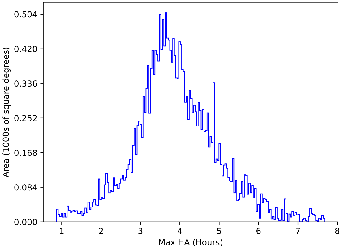
too_10_1v3.4_10yrs All sky u band: Max HA
