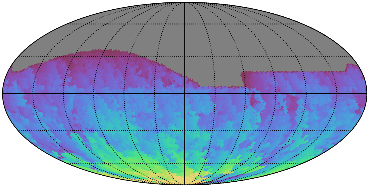
too_10_1v3.4_10yrs All sky r band: Max HA
