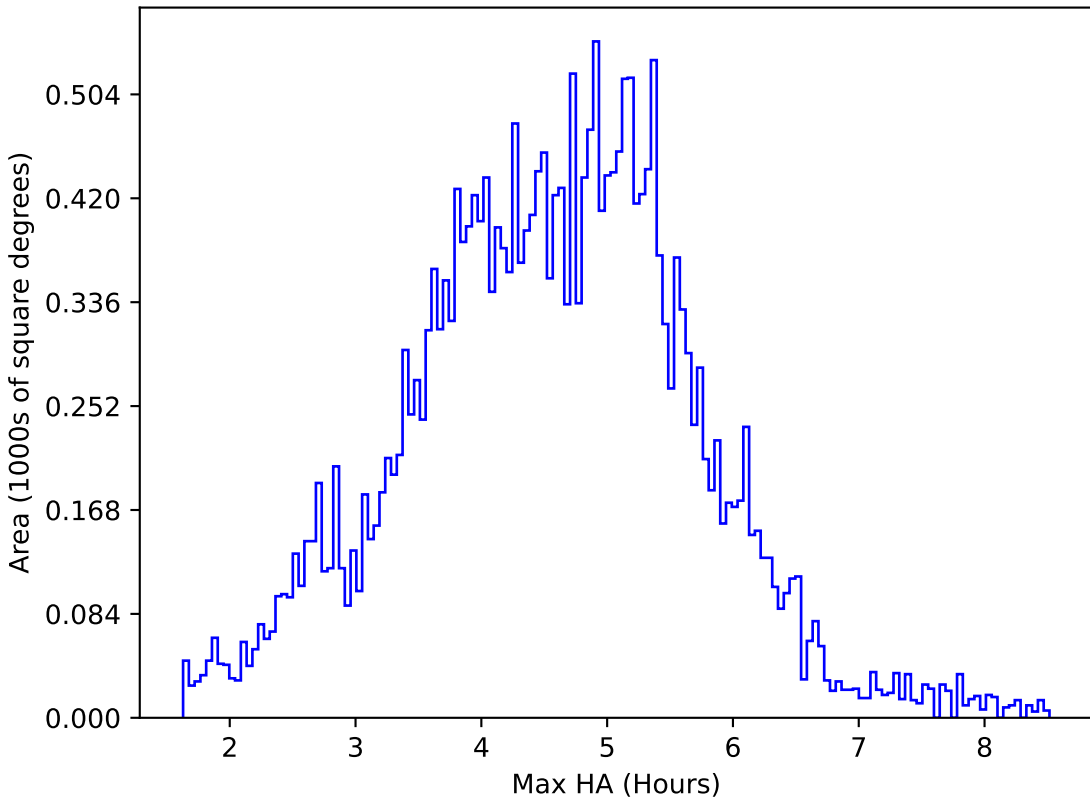
too_10_1v3.4_10yrs All sky i band: Max HA
