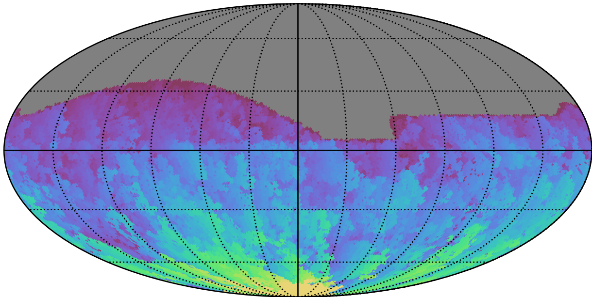
too_10_1v3.4_10yrs All sky g band: Max HA
