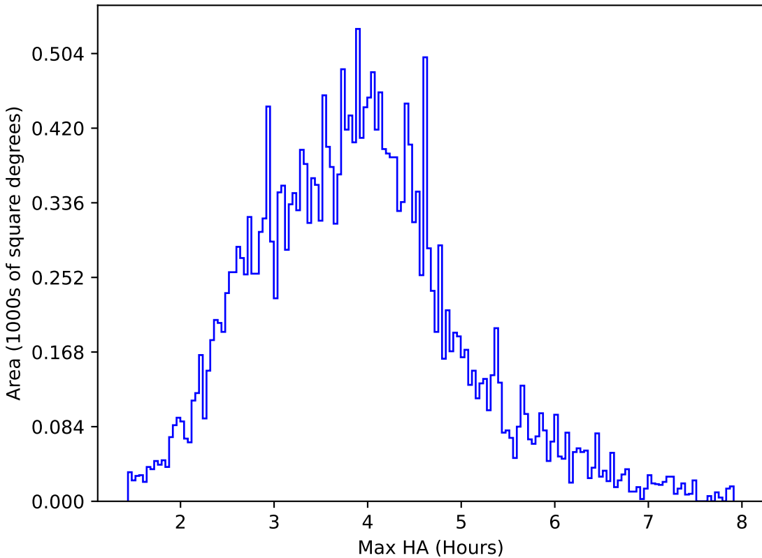
too_10_1v3.4_10yrs All sky g band: Max HA
