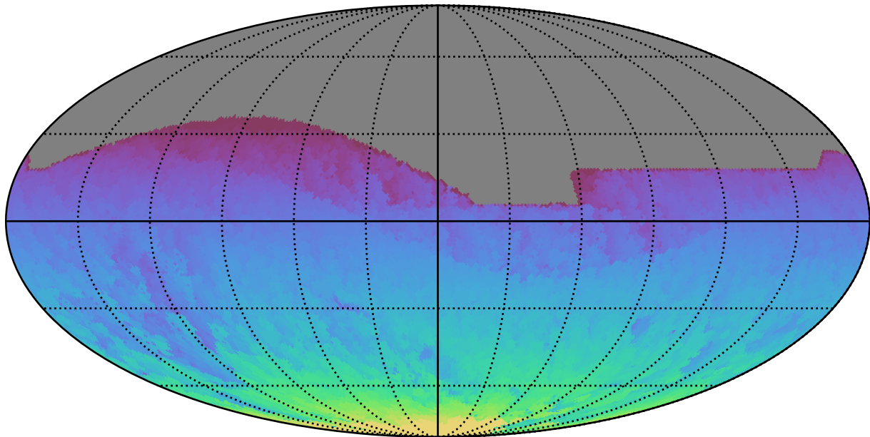
too_10_1v3.4_10yrs All sky all bands: Max HA
