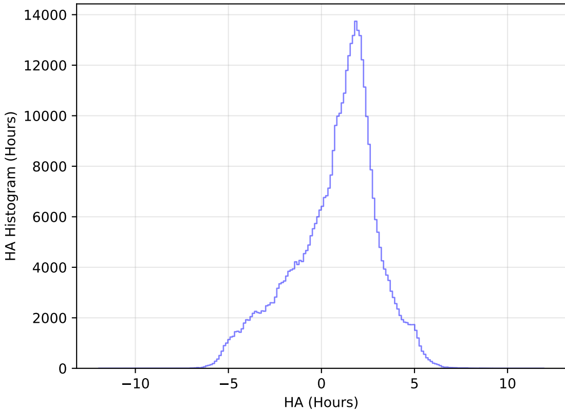
too_10_1v3.4_10yrs WFD z band: HA Histogram
