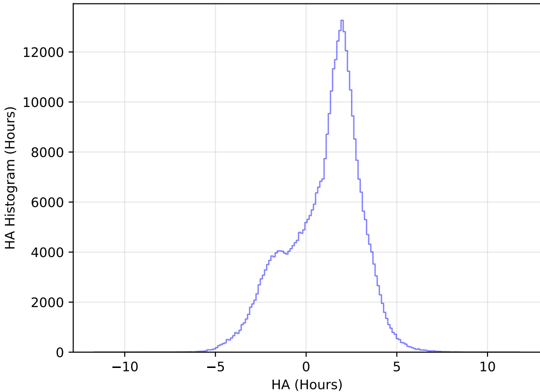
too_10_1v3.4_10yrs WFD y band: HA Histogram
