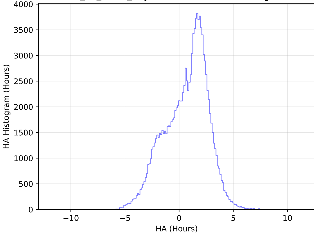
too_10_1v3.4_10yrs WFD u band: HA Histogram
