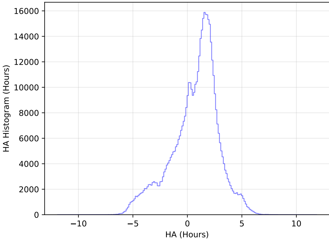
too_10_1v3.4_10yrs WFD i band: HA Histogram
