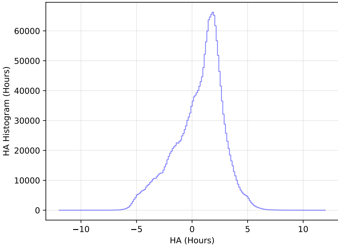
too_10_1v3.4_10yrs WFD all bands: HA Histogram
