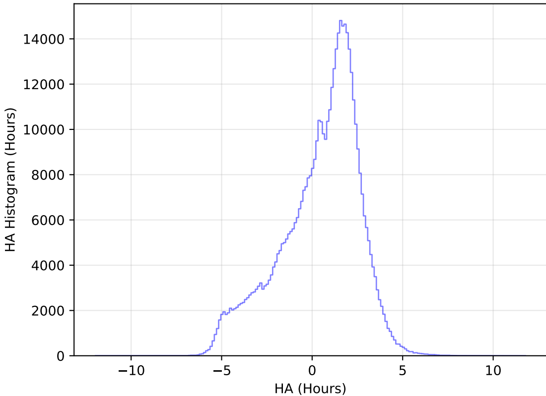
too_10_1v3.4_10yrs All sky r band: HA Histogram
