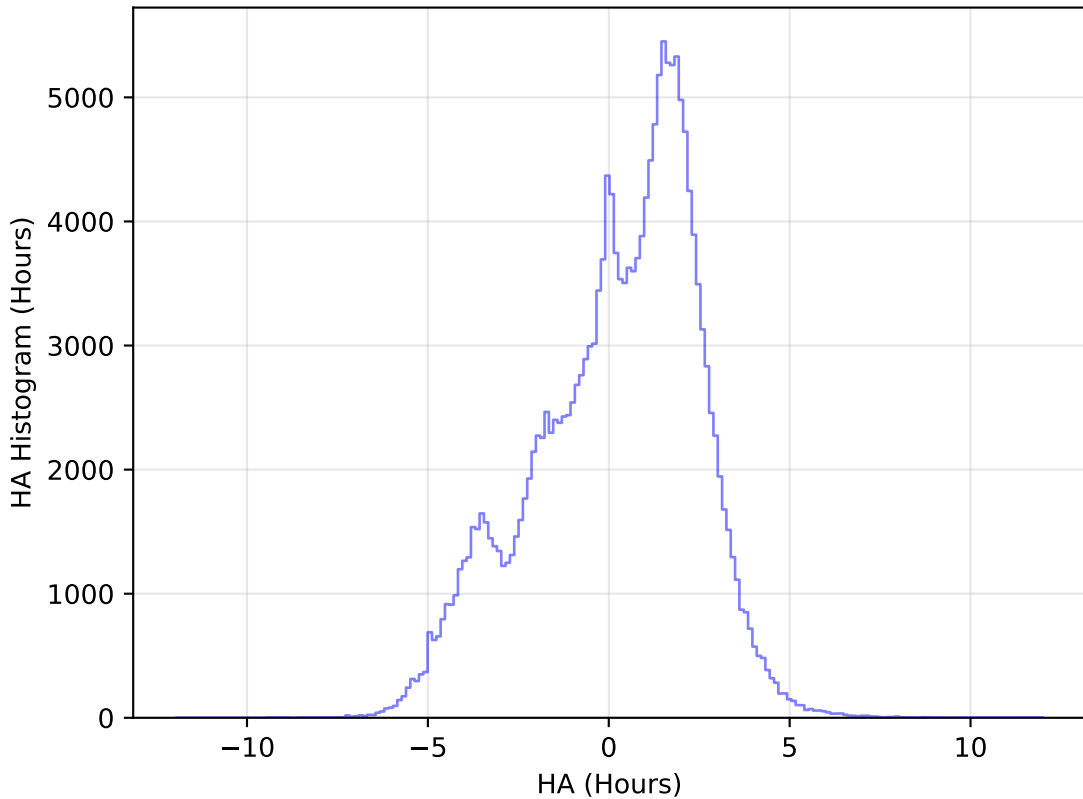
too_10_1v3.4_10yrs All sky g band: HA Histogram
