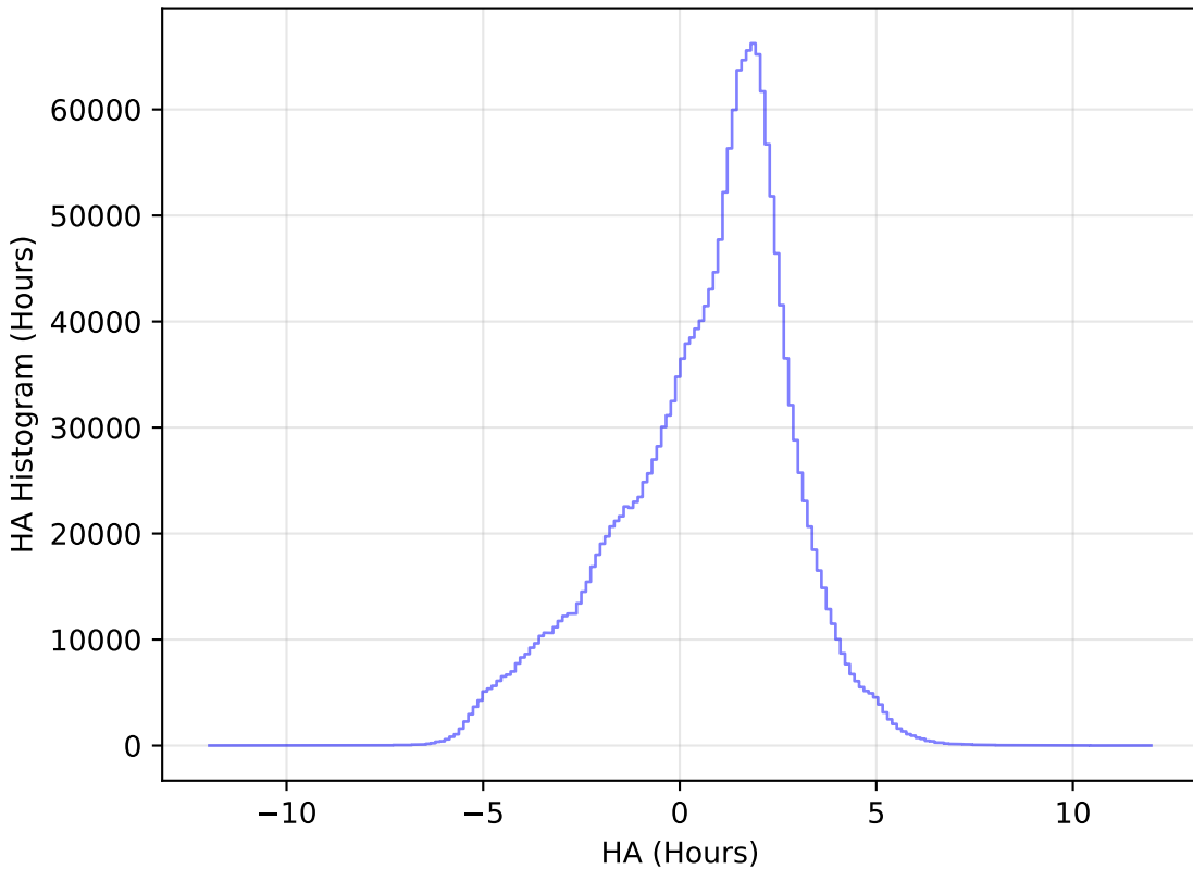
too_10_1v3.4_10yrs All sky all bands: HA Histogram
