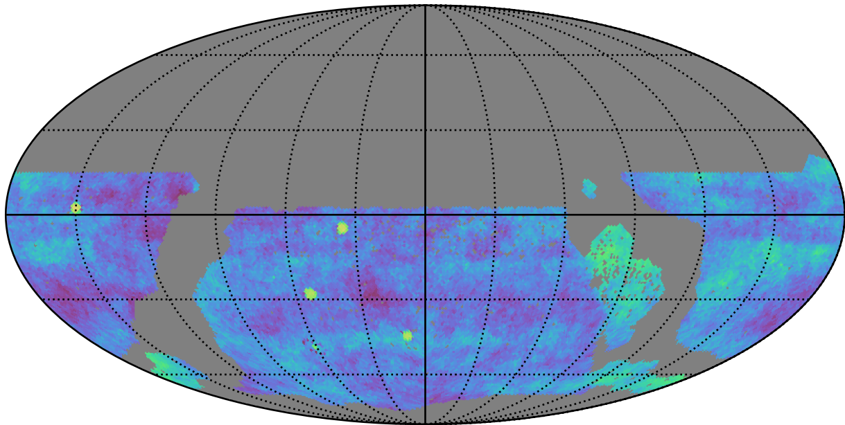
too_10_1v3.4_10yrs gri WFD: Fraction of visits in pairs (20-90 min)
