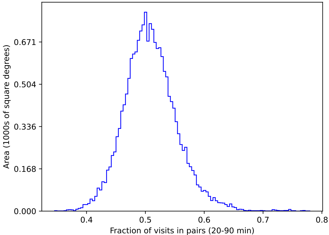
too_10_1v3.4_10yrs gri WFD: Fraction of visits in pairs (20-90 min)
