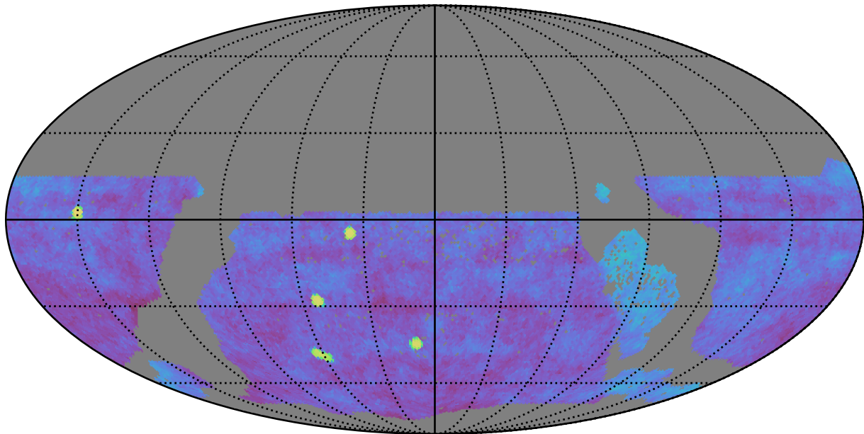
too_10_1v3.4_10yrs gri WFD: Fraction of visits in pairs (10-60 min)
