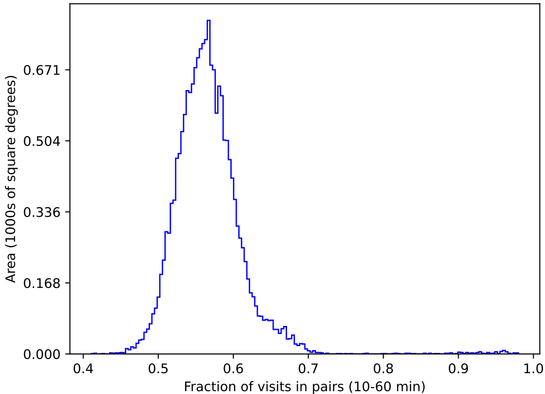
too_10_1v3.4_10yrs gri WFD: Fraction of visits in pairs (10-60 min)
