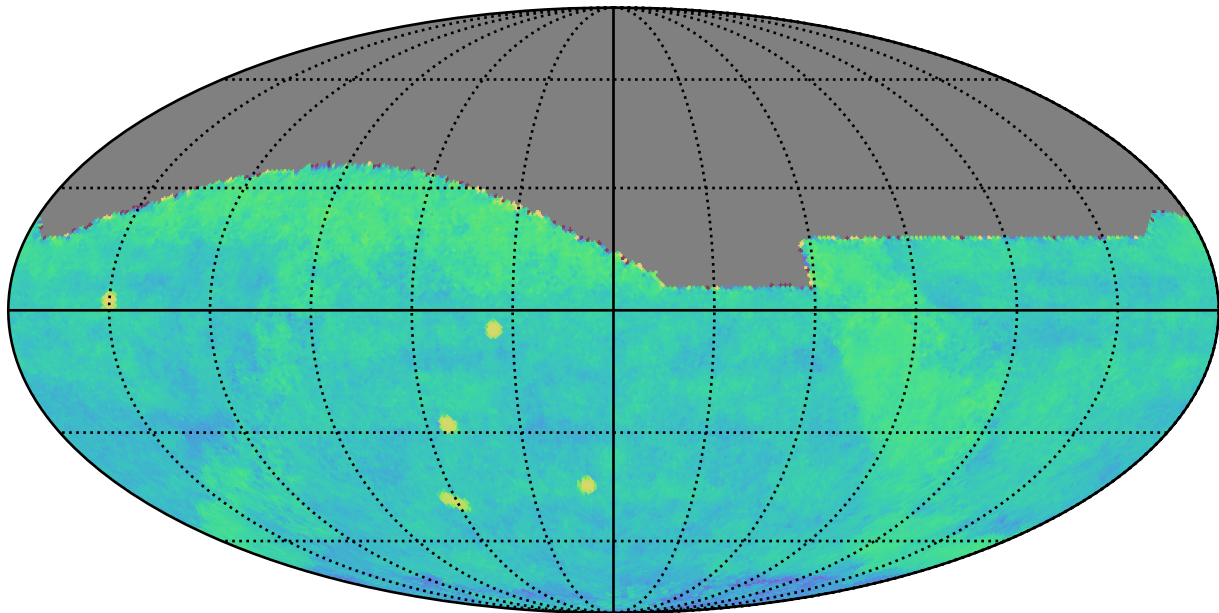
too_10_1v3.4_10yrs gri All sky: Fraction of visits in pairs (10-60 min)
