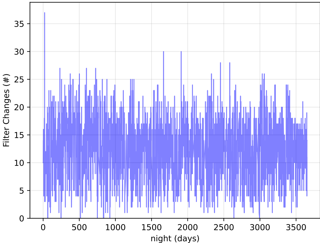
too_10_1v3.4_10yrs Per Night: Filter Changes
