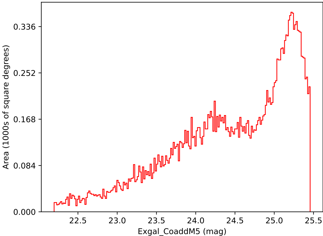
too_10_1v3.4_10yrs Yr 3-4 i band: Exgal_CoaddM5
