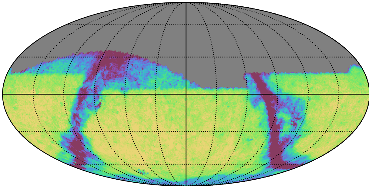
too_10_1v3.4_10yrs Yr 1 z band: Exgal_CoaddM5
