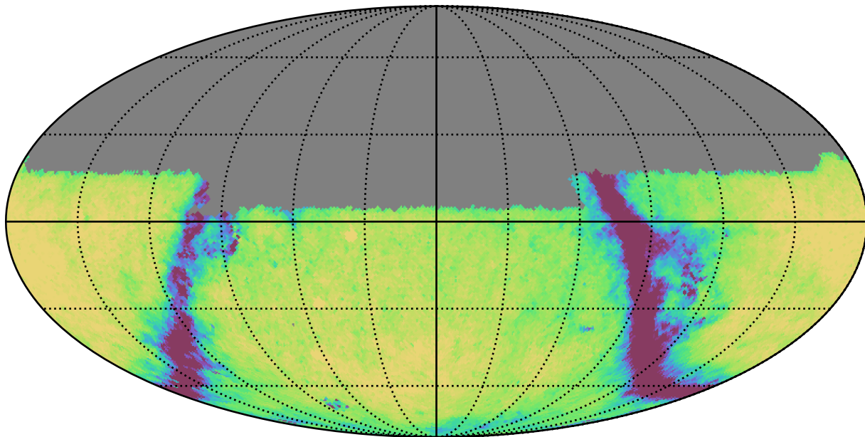
too_10_1v3.4_10yrs Yr 1 u band: Exgal_CoaddM5
