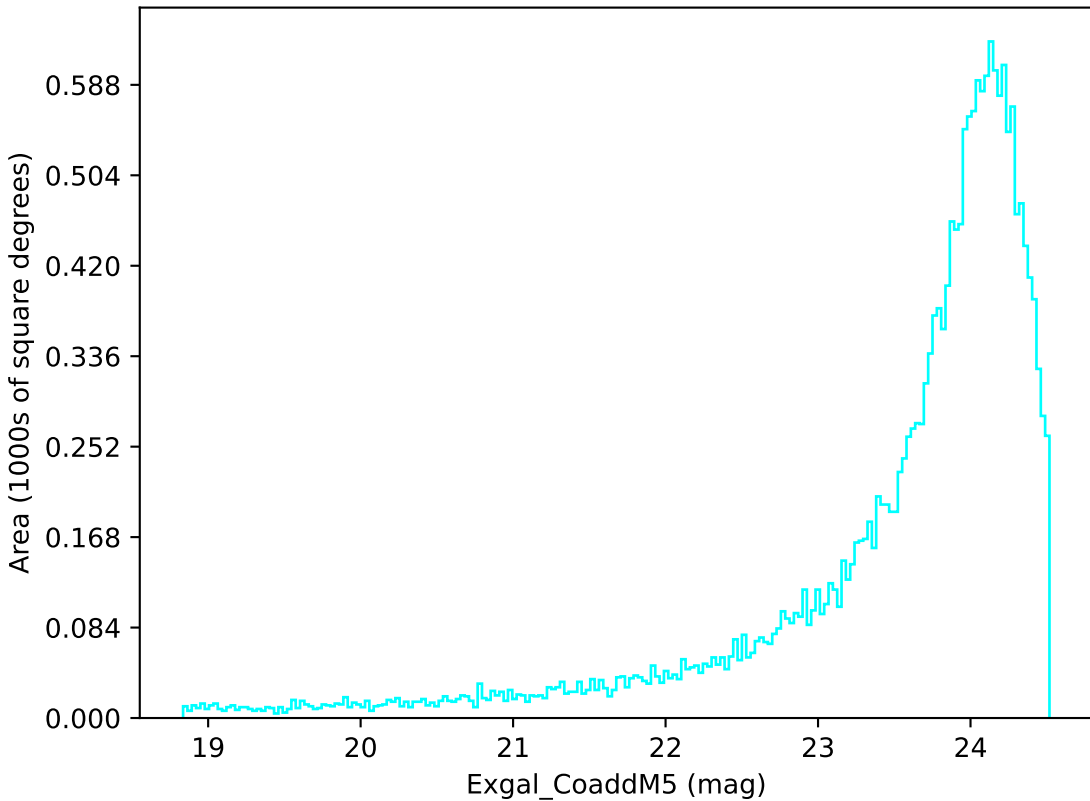
too_10_1v3.4_10yrs Yr 1 u band: Exgal_CoaddM5
