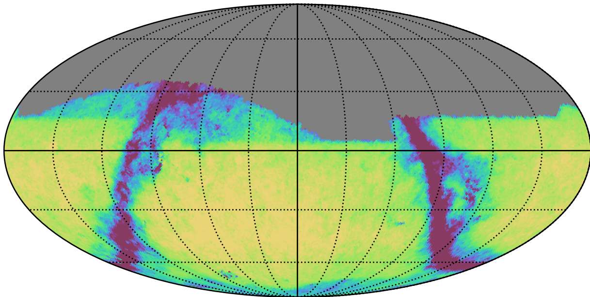
too_10_1v3.4_10yrs Yr 1 r band: Exgal_CoaddM5
