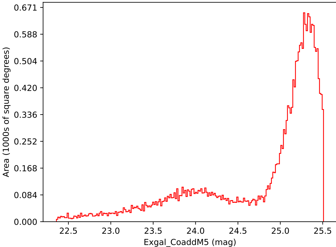
too_10_1v3.4_10yrs Yr 1 i band: Exgal_CoaddM5
