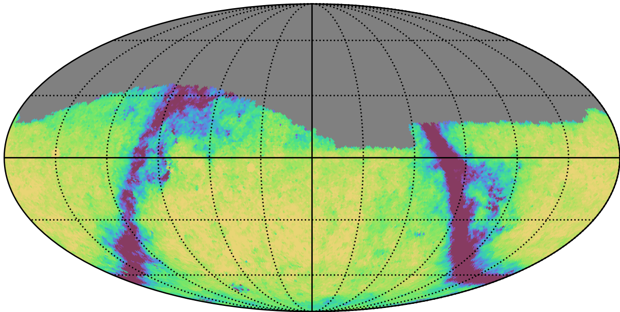
too_10_1v3.4_10yrs Yr 1 g band: Exgal_CoaddM5
