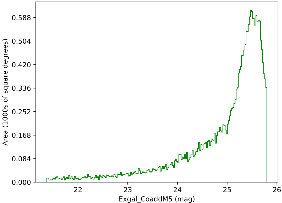
too_10_1v3.4_10yrs Yr 1 g band: Exgal_CoaddM5
