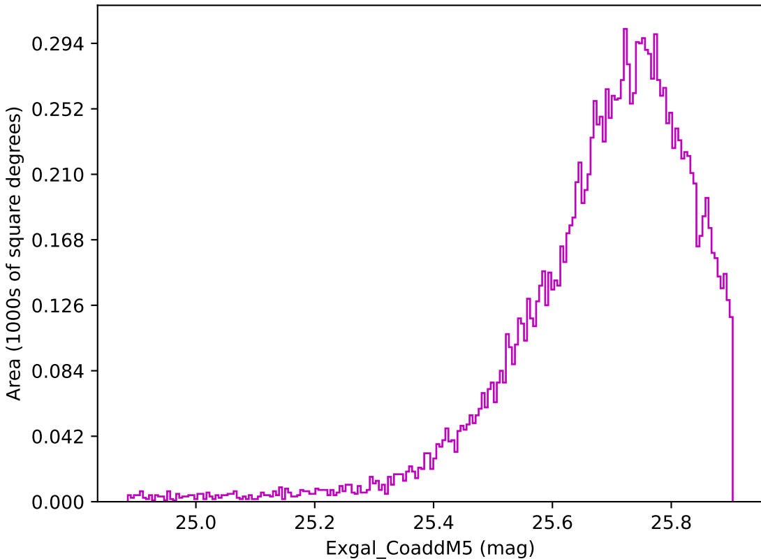
too_10_1v3.4_10yrs WFD z band: Exgal_CoaddM5
