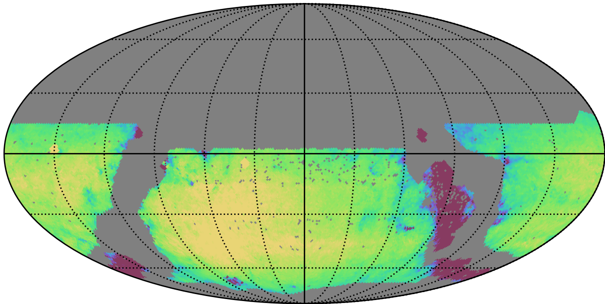
too_10_1v3.4_10yrs WFD r band: Exgal_CoaddM5
