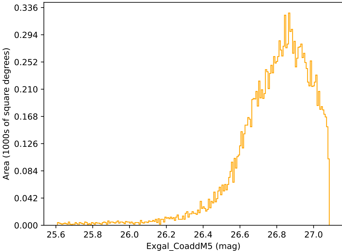
too_10_1v3.4_10yrs WFD r band: Exgal_CoaddM5
