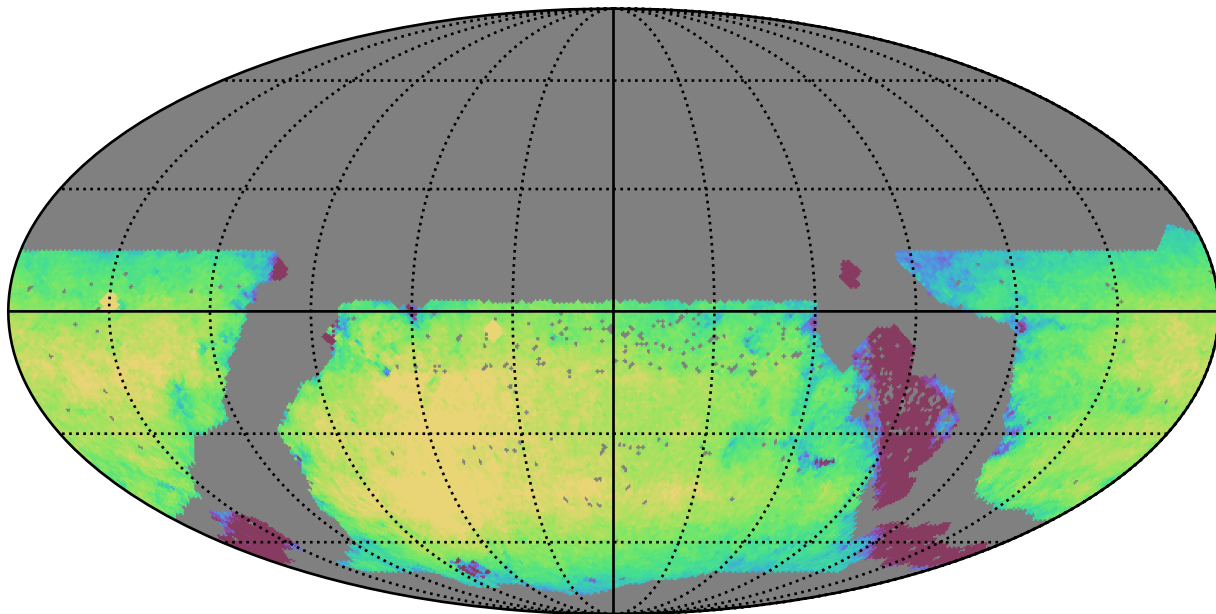
too_10_1v3.4_10yrs WFD i band: Exgal_CoaddM5
