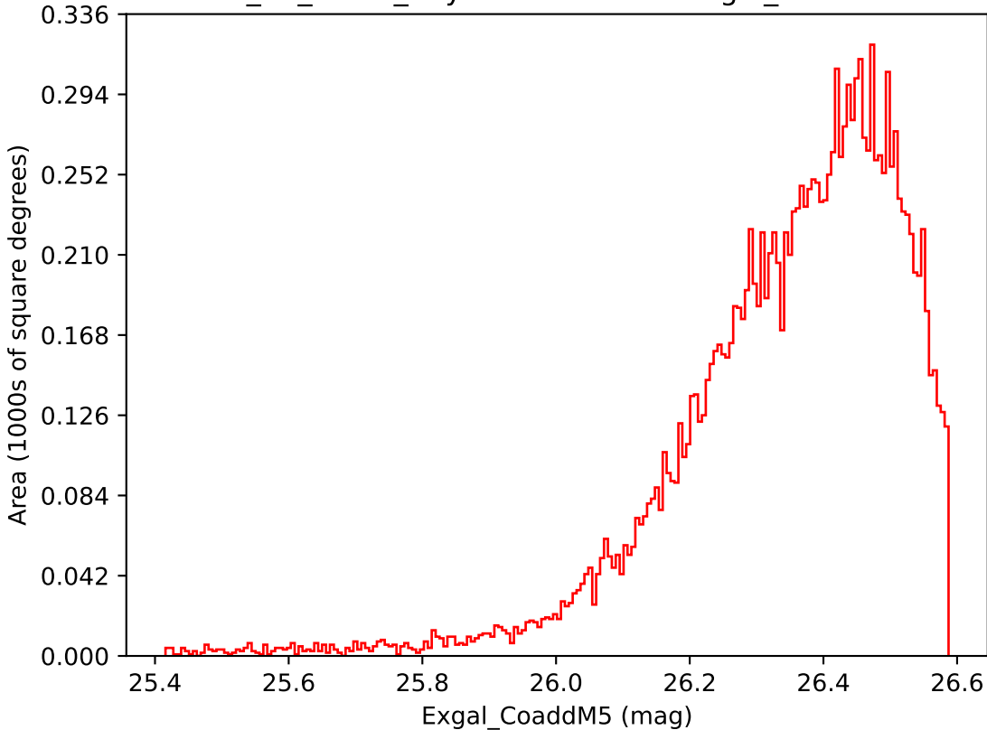
too_10_1v3.4_10yrs WFD i band: Exgal_CoaddM5
