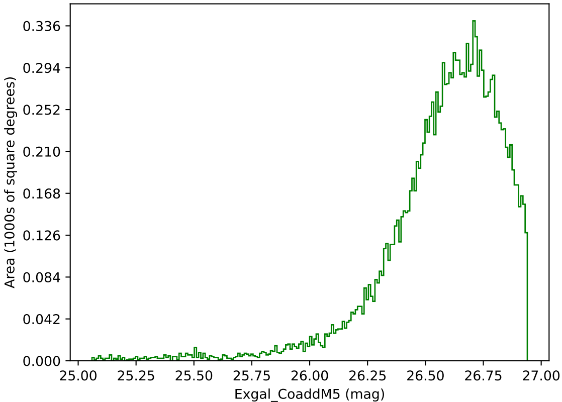
too_10_1v3.4_10yrs WFD g band: Exgal_CoaddM5
