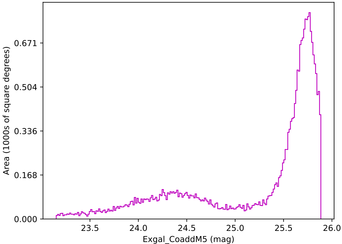
too_10_1v3.4_10yrs All sky z band: Exgal_CoaddM5
