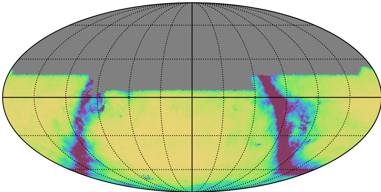
too_10_1v3.4_10yrs All sky u band: Exgal_CoaddM5
