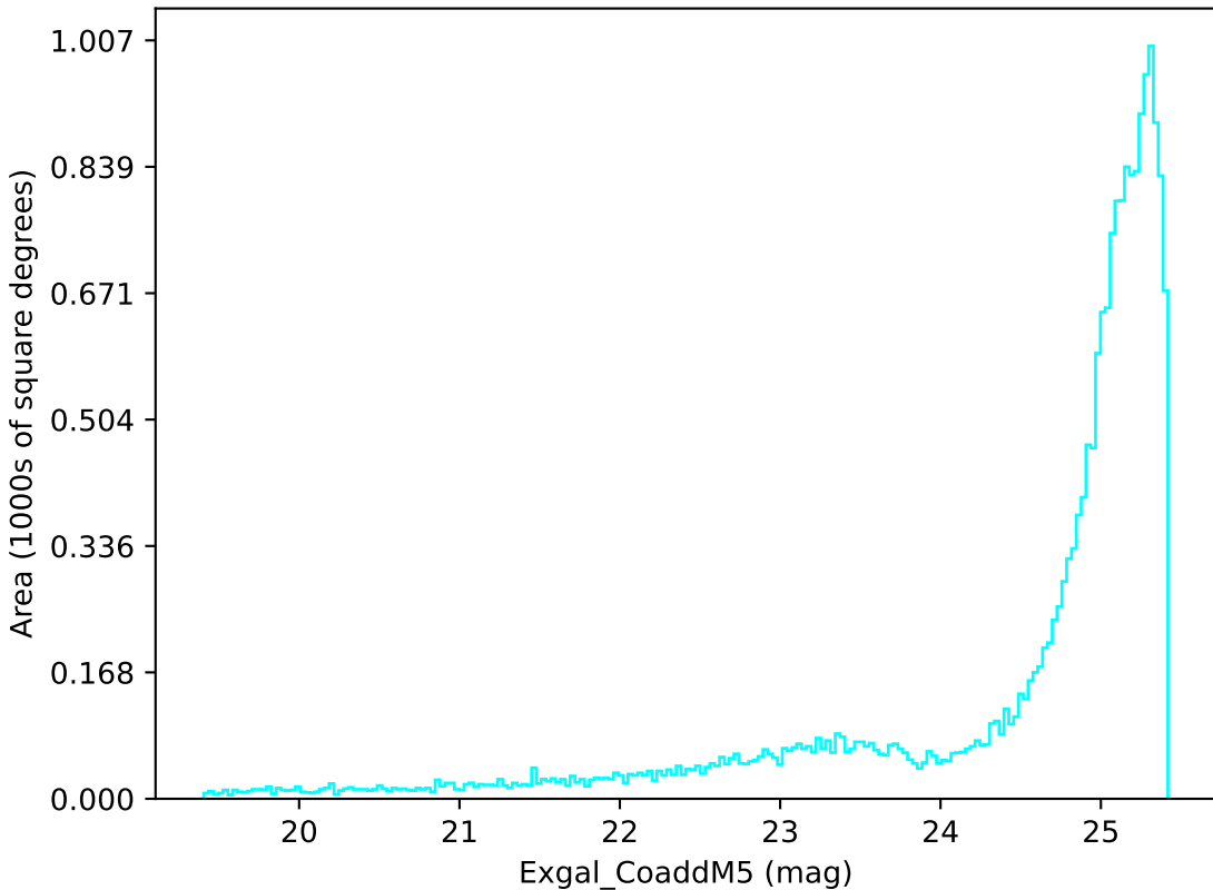
too_10_1v3.4_10yrs All sky u band: Exgal_CoaddM5
