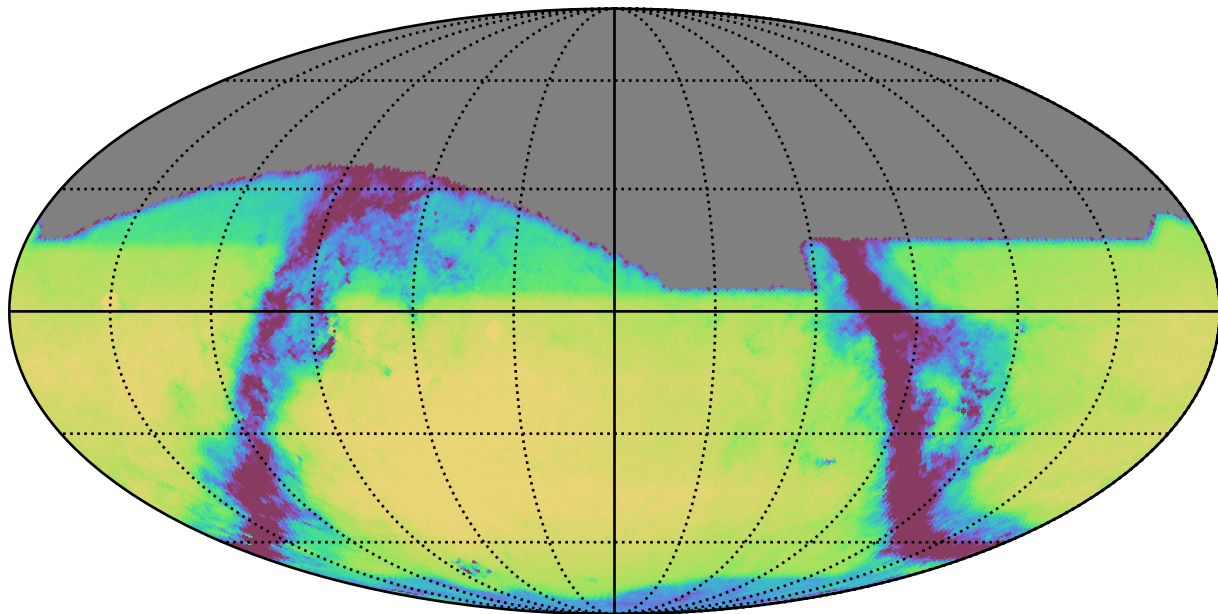
too_10_1v3.4_10yrs All sky r band: Exgal_CoaddM5
