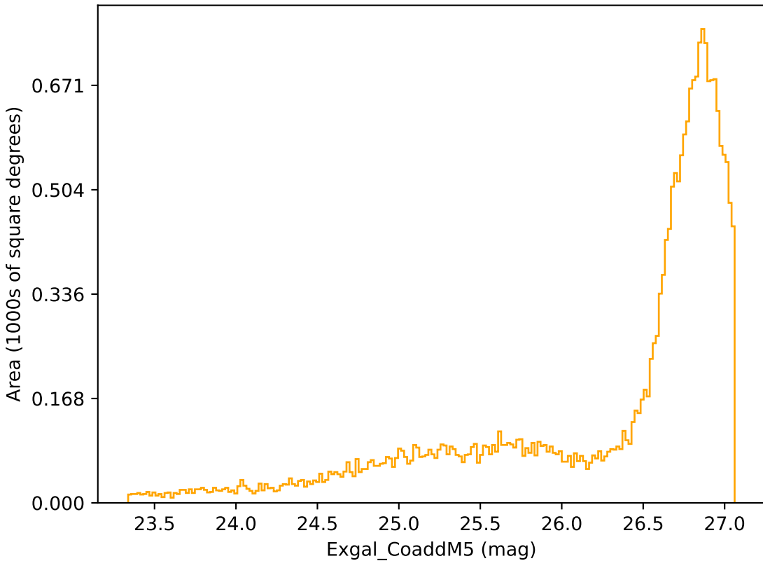
too_10_1v3.4_10yrs All sky r band: Exgal_CoaddM5
