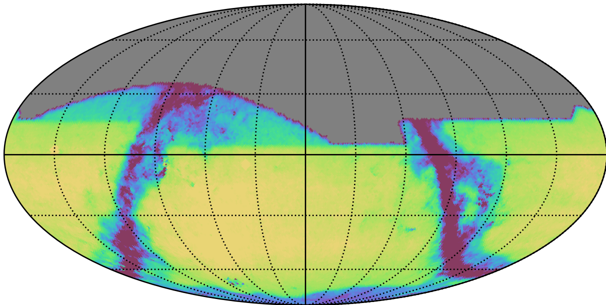
too_10_1v3.4_10yrs All sky i band: Exgal_CoaddM5
