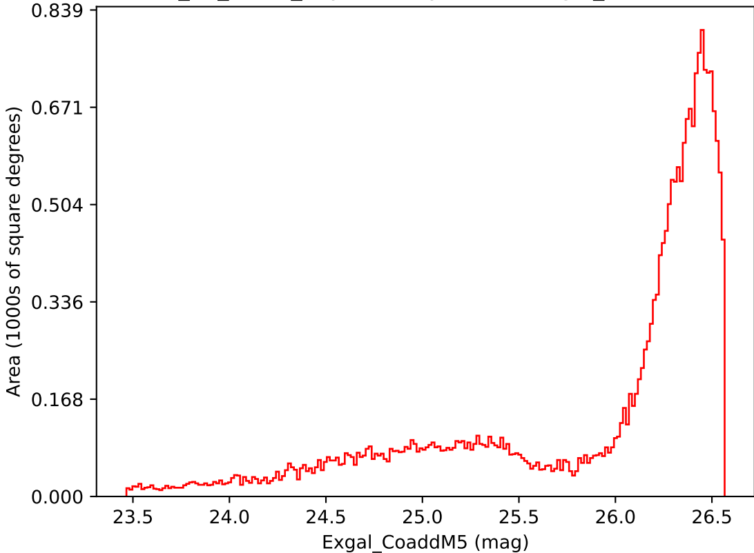
too_10_1v3.4_10yrs All sky i band: Exgal_CoaddM5
