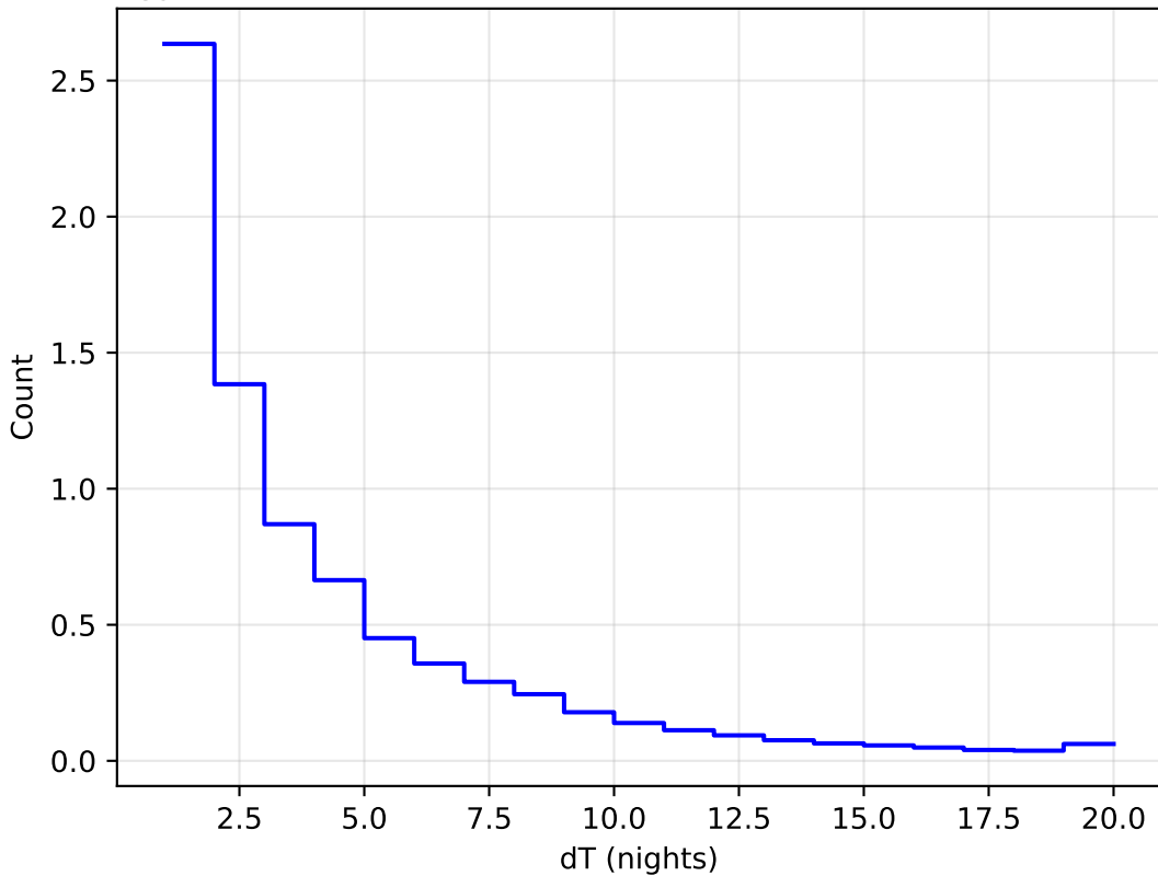
too_10_1v3.4_10yrs WFD all bands: DeltaNight Histogram 1e6
