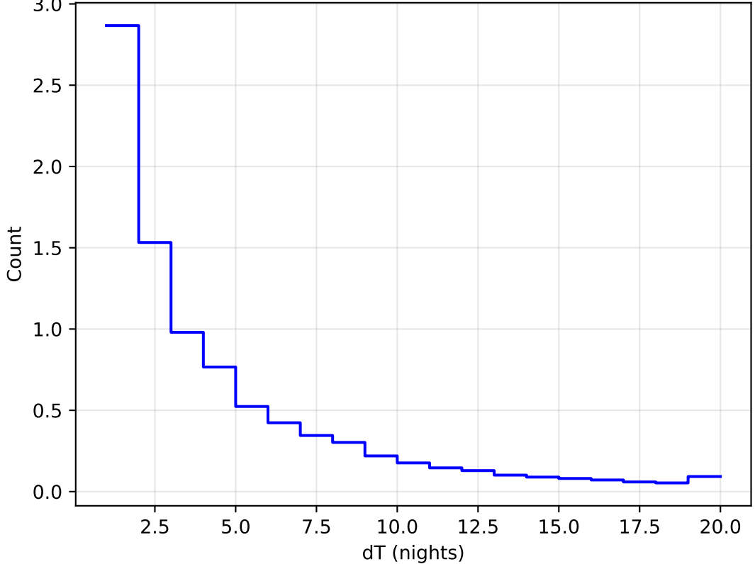
too_10_1v3.4_10yrs All sky all bands: DeltaNight Histogram 1e6
