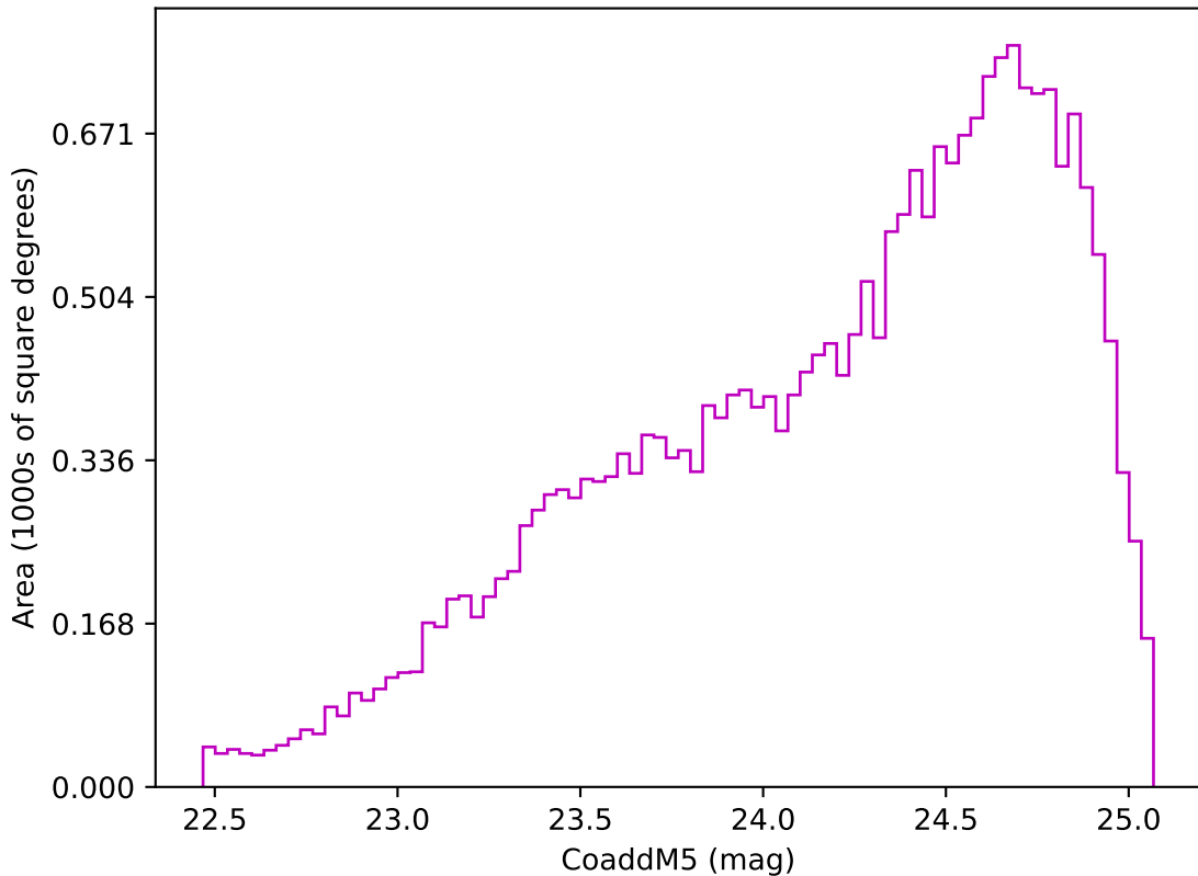
too_10_1v3.4_10yrs Yr 3-4 z band: CoaddM5
